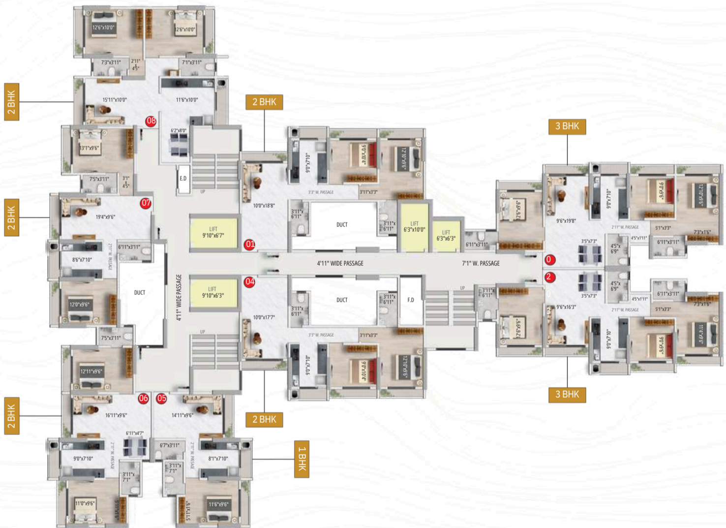
TYPICAL 3RD TO 22ND FLOOR | REFUGEE 8TH, 12TH, 16TH & 20TH
